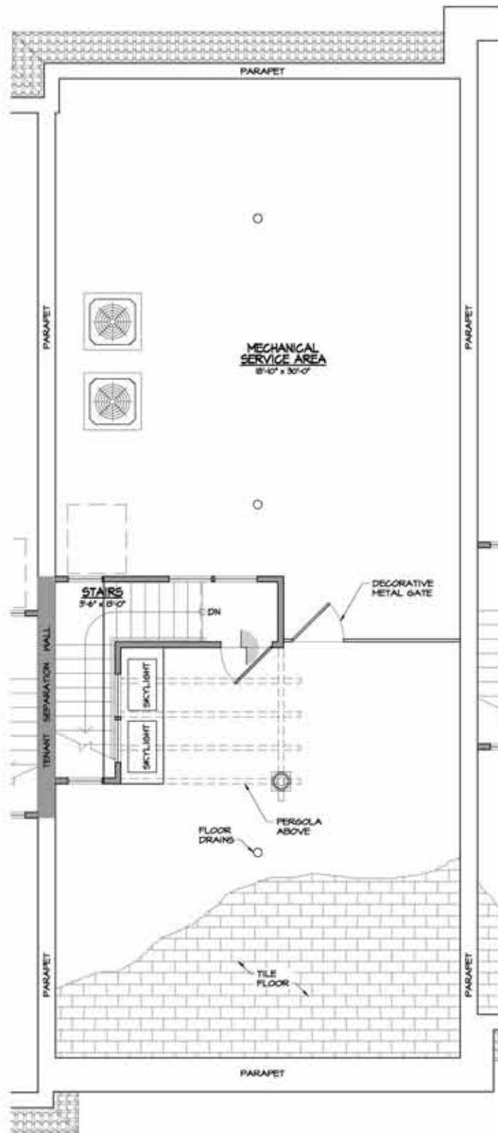
TYPICAL UNIT ROOF TERRACE PLAN
