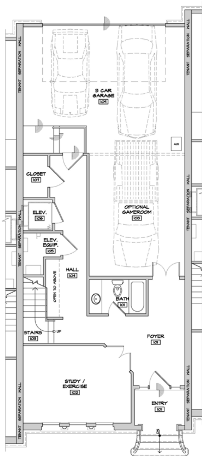
TYPICAL UNIT FIRST FLOOR PLAN
