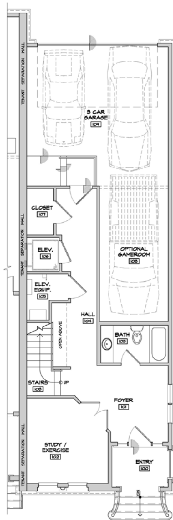
END UNIT FIRST FLOOR PLAN
